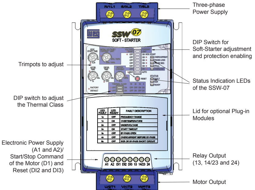
Figure 2.1 - Frontal view of the SSW-07
