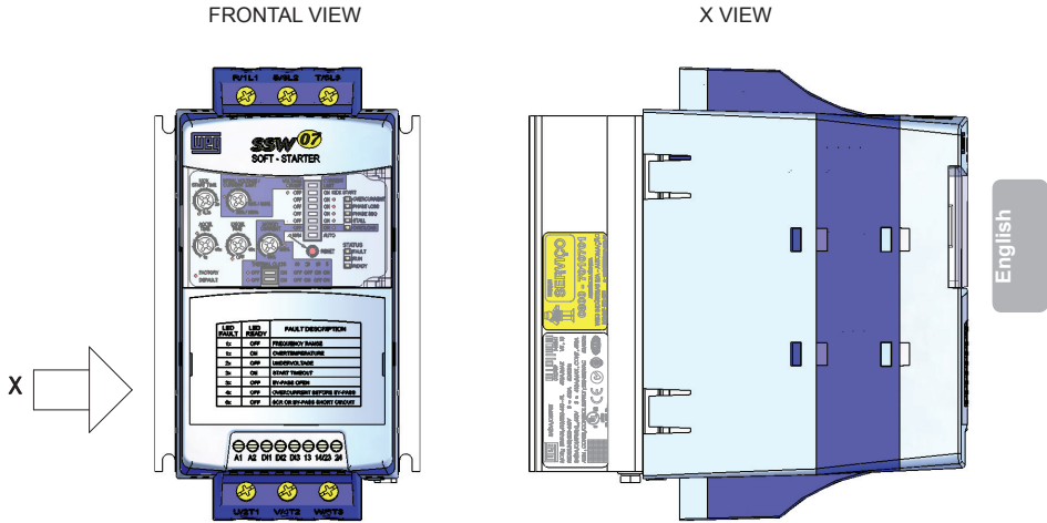
Figure 2.4 - Location of the labels
