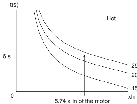
Figure 5.8 - Checking of the maximum thermal class, considering the S.F.
