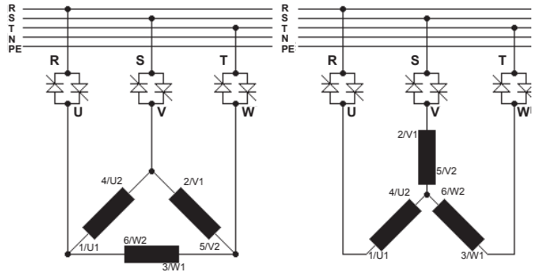
Figure 3.7 - Soft-Starter SSW-07 with standard connection
