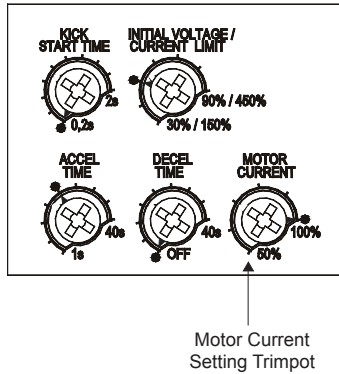
Figure 4.7 - Motor current setting
