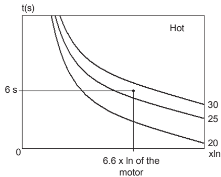
Figure 5.7 - Checking the maximum class of curves in hot condition
