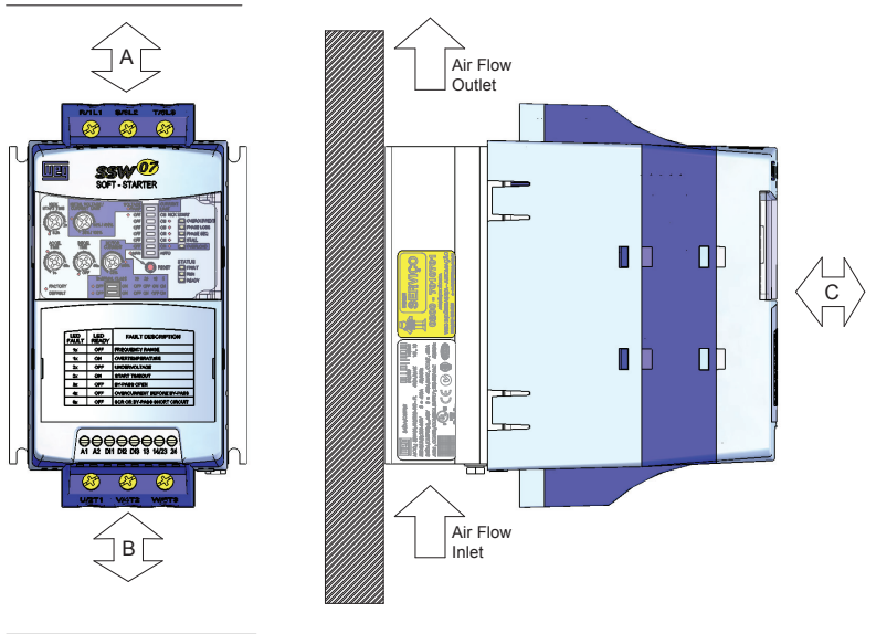
Figure 3.2 - Free spaces for ventilation
