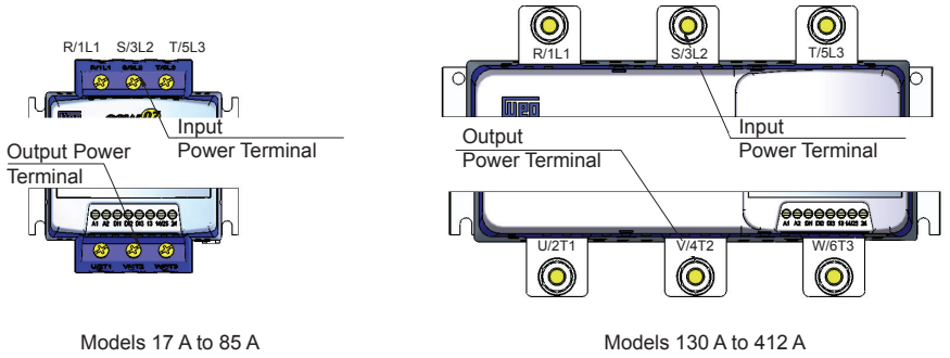
Figure 3.5 - Power terminals
