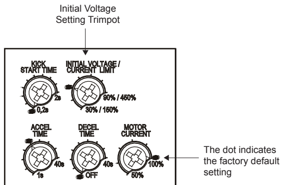
Figure 4.3 - Initial voltage setting
