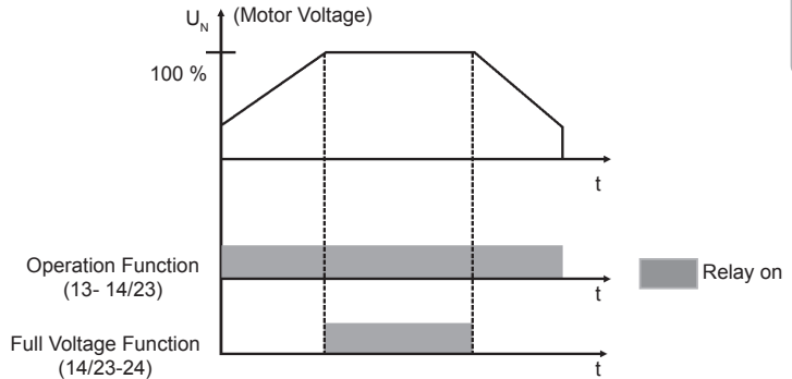
Figure 4.11 - Output relay operation
