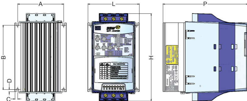
Figure 3.1 - SSW-07 dimensions
