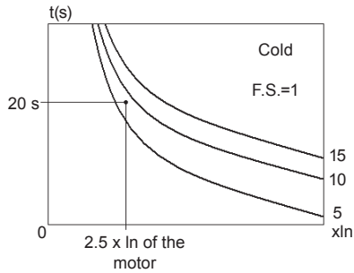
Figure 5.6 - Checking the minimum class of curves in cold condition
