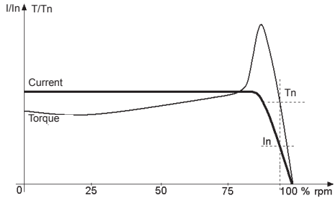
Figure 5.2 - Characteristic curves of torque and current in a current limitation start
