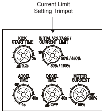
Figure 4.4 - Current limit setting
