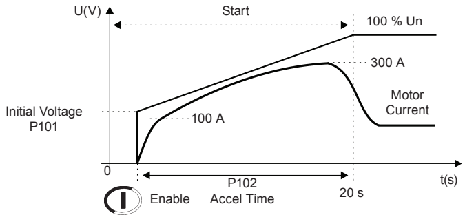
Figure 5.5 - Typical current curve during a voltage ramp start
