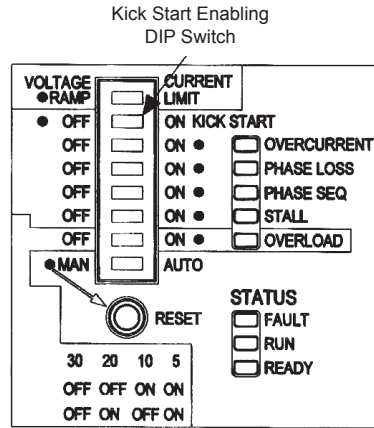
Figure 4.2 - Kick Start enabling
