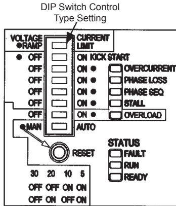
Figure 4.1 - Control type setting
